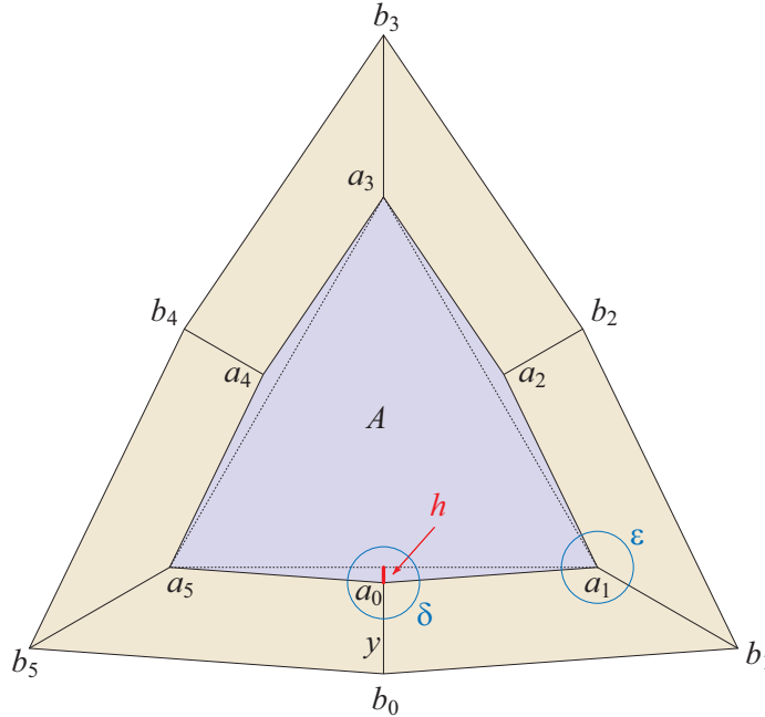
Figure 2: Overhead view of prismatic. If an origin is set at the midpoint of the bottom side of the equilateral triangle on A , then a_0 = (0, -h, 0) and b_0 = (0, -(h + y), -z) .
