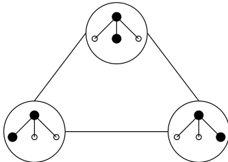
FIGURE 2. X_2(K_{1,3}) .
