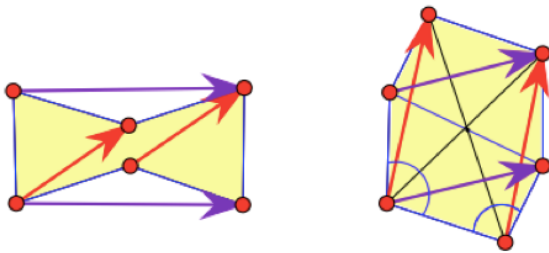
Figure 17: For the ‘reentrant’ structure of hexagons in Figure 5, which has two degrees-of-freedom, the figure on the right marks two angles which may be used as parameters. By maintaining the central symmetry of the hexagon, the two depicted pairs of periods remain equal vectors.
