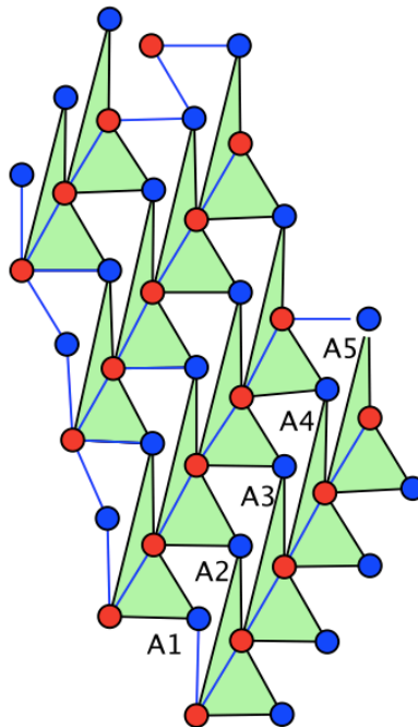
Figure 18: An ultrarigid framework obtained from a periodic pseudo-triangulation with an additional edge orbit. When ignoring periodicity, finite fragments are flexible.
