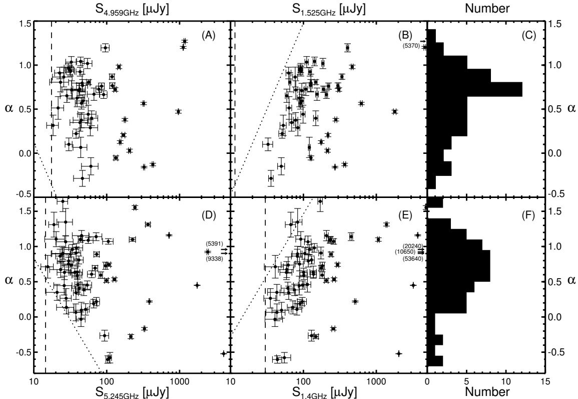
Figure 4. Radio spectral index as a function of flux density. The radio spectral indices of our 5 GHz radio sources are plotted as functions of flux densities at 5.0 GHz (panel A), 1.5 GHz (panel B) for the GN field, and 5.2 GHz (panel D) and 1.4 GHz (panel E) for the GS field with 5\sigma flux limits of each survey (dashed line), i.e. 17.5\mu\text{Jy} (A), 11.5\mu\text{Jy} (B), 15\mu\text{Jy} (D), and 30\mu\text{Jy} (E). The sources located outside the panels are marked with arrows, and their flux densities are given inside the parentheses. The dotted line in each panel represents the sensitivity of radio spectral index limited by the survey limit of adjacent survey. Histograms of SI distribution for the GN and GS fields are shown in panels (C) and (F), respectively.
