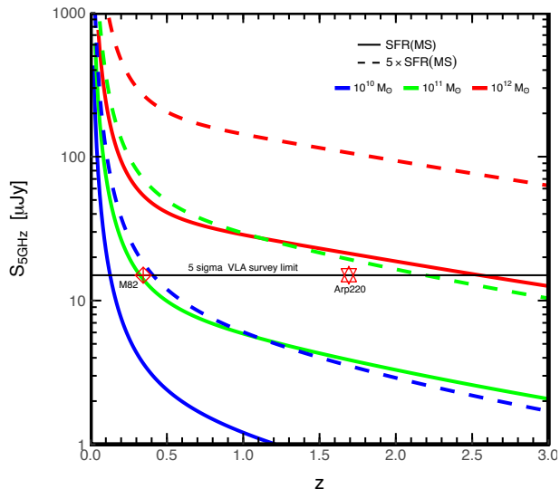
Figure 9. Detectability of MS SFGs and a sensitivity of radio observations. We show the observable galaxies with a certain SFR and stellar mass as a function of redshift. We show SFGs with SFR of MS (solid lines) and 5\times SFR of MS (dashed lines) as a function of redshift with respect to the stellar masses of 10^{10}M_{\odot} (blue), 10^{11}M_{\odot} (green), and 10^{12}M_{\odot} (red). The survey limits ( 5\sigma ) of our radio observations are indicated by the horizontal lines, i.e. 15\mu\text{Jy} for GS. As examples, we marked the maximum redshifts of detecting M82-like (red diamond) and Arp220-like (red star) galaxies at the survey limits.
