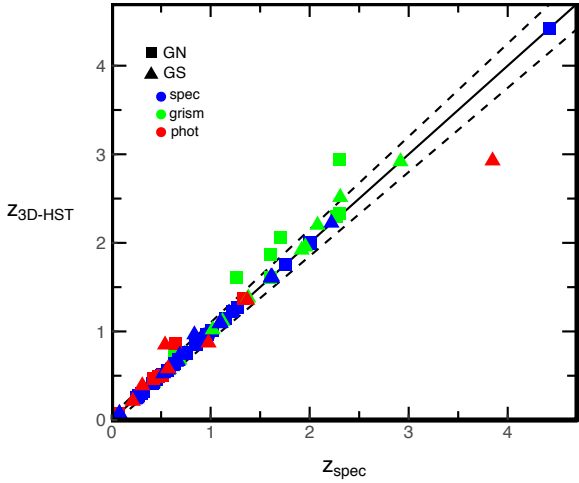
Figure 2. Comparison of our spectroscopic redshifts and the best redshifts in 3D-HST for the GN (square) and the GS (triangle) fields. The color represents the type of redshift measurements, e.g. spectroscopy (blue), grism (green), and photometry (red). The solid line is the one-to-one line and dashed lines show the selection limits of \pm 0.05 in |z_{\text{spec}} - z_{\text{best},3D-HST}|/(1 + z_{\text{spec}}) < 0.05 .
