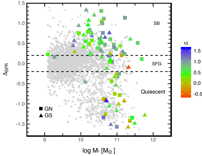
Figure 6. Offset of SFR from the MS ( \Delta_{SFR} ) and stellar mass with a color code according to radio spectral index in GN (squares) and GS (triangles) fields. Small gray points are the 3D-HST galaxies without radio counterparts in GN and GS fields for a comparison. The dashed lines of \Delta_{SFR} = \pm 0.2 indicate the selection of SFGs. SBs are sources above a line of \Delta_{SFR} > 0.2 while quiescent galaxies are those below a line of \Delta_{SFR} < -0.2 . The distribution of radio spectral index show that SFG+SB have mainly steep spectra while quiescent galaxies have flatter spectra even though both have wide distributions.
