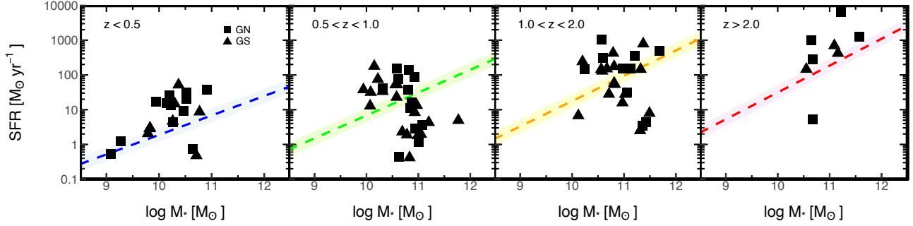
Figure 5. The SFR and stellar mass distributions of the GS and GN radio sources with respect to the MS in four redshift bins. We represent the SFR and stellar mass distribution of radio sources in GN (squares) and GS (triangles) in four redshift bins, z < 0.5 , 0.5 < z < 1.0 , 1.0 < z < 2.0 , and z > 2.0 . A dashed lines show the SFR-stellar mass relation of the MS at mean redshifts 0.25 (blue), 0.75 (green), 1.5 (orange), and 2.5 (red) with dispersion of \pm 0.2 (shaded regions).
