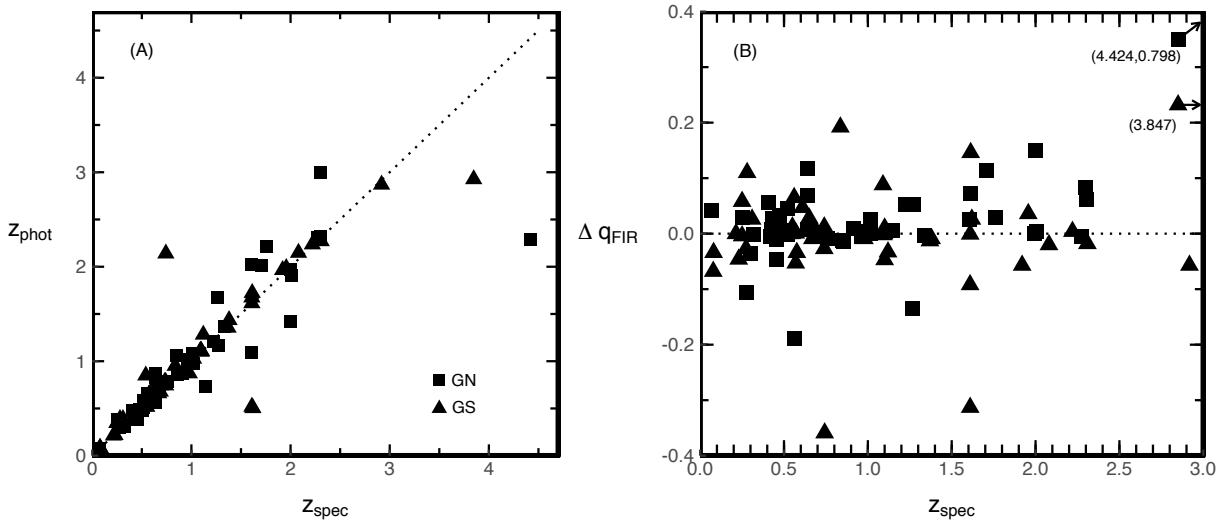
Figure 13. Comparison of the photometric and spectroscopic redshifts from the 3D-HST project (left panel) and the resulting error in the radio-FIR correlation parameter ( \Delta q_{FIR} ) as a function of spectroscopic redshift (right panel). The additional scatter in \Delta q_{FIR} resulting from using photometric redshift is 0.112 in dex.
