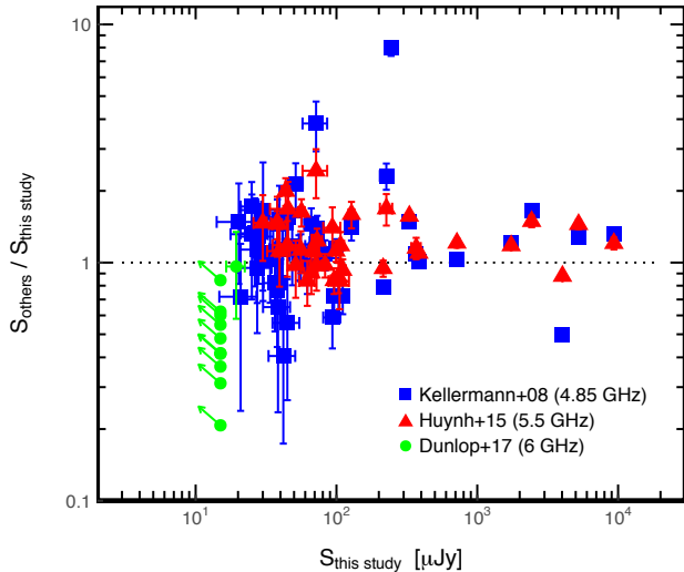
Figure 10. Measured flux density comparison among the radio sources in the GS field with those reported by previous studies with different angular resolution. Those by Kellermann et al. (2008) and Huynh et al. (2015) with \sim 3 times larger beams are on average \sim 30 percent larger. The higher resolution survey by Rujopakarn et al. (2016) with 0.61'' \times 0.31'' beam has only one detected source in common (the 6 GHz source flux densities are actually reported by Dunlop et al. 2017) that agrees well with ours. The dotted line is the unity ratio line to guide the eye.
