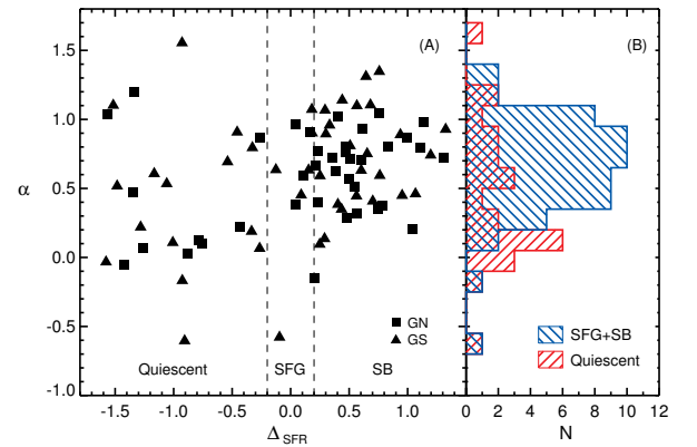
Figure 7. Radio spectral index distribution as a function of \Delta_{SFR} . The panel (A) shows that the radio spectral index distribution of SFG+SB ( \Delta_{SFR} > -0.2 ) is more tightly clustered around \alpha \sim 0.8 , in comparison with the quiescent galaxies ( \Delta_{SFR} < -0.2 ), which are distributed more uniformly and widely in spectral index \alpha . These trends are easily seen in the histograms of SFG+SB (blue) and quiescent galaxies (red) in panel (B). The Kolmogorov-Smirnov test indicates that the radio spectral index distributions of the two populations are different from each other with a p-value of 0.0015.
