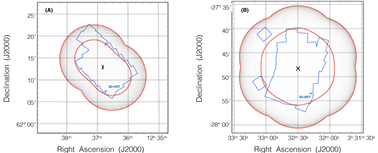
Figure 1. The VLA 5 GHz mosaic images for the GN (panel A) and the GS (panel B) fields. The inner red contours trace the boundary where the primary beam correction increases the effective noise to twice that in the image center, and this also marks the survey area where the source catalogs are derived. The outer red contours mark the survey areas where the primary beam response is 7% of the mosaic center. The centers of each mosaic are marked with a cross ('x'), and the 3D-HST coverages are outlined in blue polygons.
