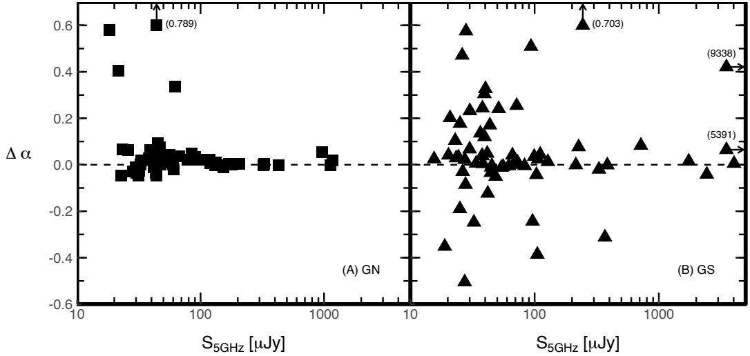
Figure 11. Deviations of radio spectral index measured without matching the beam sizes ( \alpha_{non} ) from that measured by matching beam sizes ( \alpha_{beam} ). The deviation of radio spectral index ( \Delta\alpha = \alpha_{non} - \alpha_{beam} ) is shown as a function of 5 GHz flux density for the GN field (left panel) and for the GS field (right panel). The main difference is the much larger synthesized beam for the 1.4 GHz data in the GS field.
