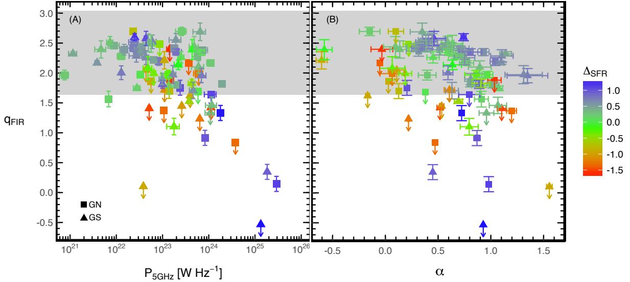
Figure 8. The radio-FIR correlation parameter ( q_{FIR} ) as a function of 5 GHz power (left panel) and radio spectral index (right panel). Radio sources in GN (squares) and GS (triangles) are plotted with the color code of \Delta_{SFR} and arrows showing the upper limits. A shaded region represents the range of q_{FIR} of local SFGs, i.e. q_{FIR} = [1.64, 3.04] (Yun et al. 2001). Most SFG+SB (with \Delta_{SFR} > -0.2 ) are located inside the region of local SFGs while most quiescent galaxies (with \Delta_{SFR} < -0.2 ) have lower q_{FIR} .
