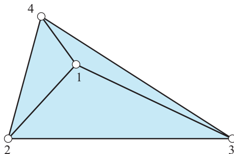
Figure 3: Triangles forming K_3 .
