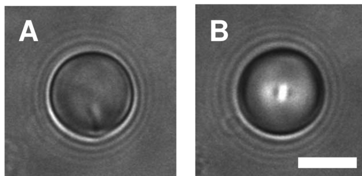
Figure 4. A) Bright-field micrograph of a polymer 1 -laden 5CB droplet freely moving above a multilayer film presenting azlactone functionality (surface 1 ). B) Bright-field micrograph of the same 5CB droplet after contacting the surface of the film (immobile). Scale bar = 5 \mu\text{m} .
