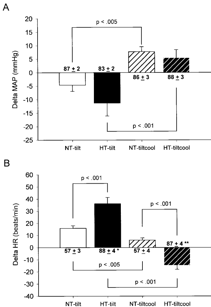
Fig. 1. Effects of tilting with and without cooling on mean arterial blood pressure (MAP; A) and heart rate (HR; B). Bars are the change (delta) in the variables between supine baseline and tilted conditions for normothermia (NT-tilt), heat stress (HT-tilt), normothermia + skin-surface cooling (NT-tilt cool ), and heat stress + skin-surface cooling (HT-tilt cool ). Numerical values associated with each bar are the values before tilting and skin cooling for that experimental condition. Values are means ± SE. *Significant differences between supine values before tilting, P < 0.001 . **Significant differences between supine values before tilting and cooling, P < 0.001 . Brackets indicate significant differences in the response that occurred with tilting, as well as the P value for that comparison.
