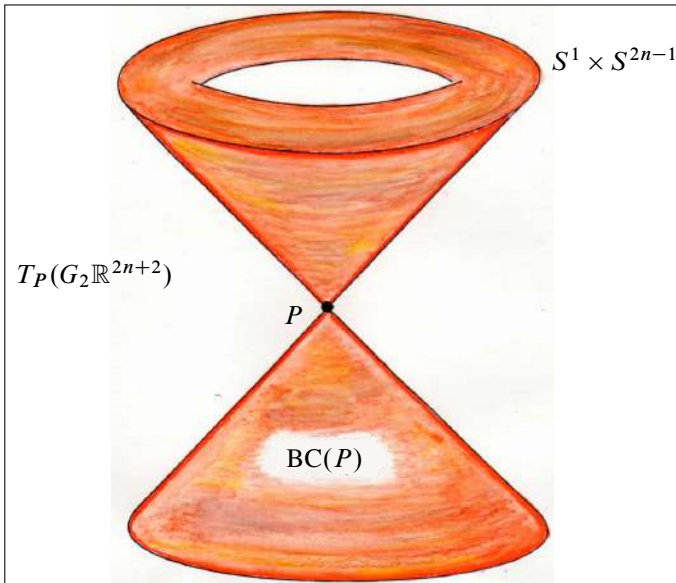
Figure 7: The bad cone \text{BC}(P)
