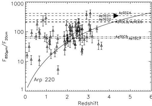
FIG. 2.— The change with redshift of the ratio of the submillimeter ( 850\mu\text{m} ) versus radio (20cm) continuum emission in SMGs (see Carilli & Yun 1999). Radio-bright SMGs with optical spectroscopic redshifts from Chapman et al. (2005) are shown as open triangles, as compared to radio-dim (dashed lines) and radio-bright (dash-dot lines) SMA/AzTEC sources (see § 4 for abbreviations). The filled triangle represents a rough redshift of z \gtrsim 4 for AzTEC1 from the B-band dropout nature of its optical counterpart. The solid line is a model track for Arp 220. SMA flux measurements at 890\mu\text{m} were corrected to 850\mu\text{m} using the F_{890\mu\text{m}}/F_{1100\mu\text{m}} ratio from SMA and AzTEC, a \lesssim 15\% correction for all the sources.
