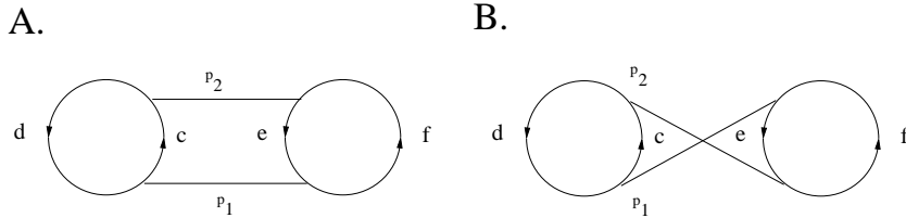
FIGURE 2. Two possible mutual positions for chords corresponding to intersection points of b_1 and b_2
