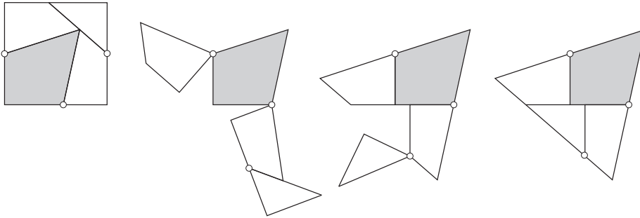
Figure 1: A four-piece hinged dissection between a square and an equilateral triangle.
