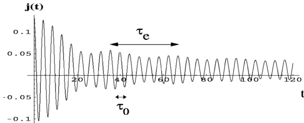
FIG. 2. Current evolution for an abrupt quench, T = 0 . We set superlattice strength V_0 = 0.7 , hopping w = 1 , and the boost \nu = \frac{\pi}{15} [i.e., initial supercurrent of j(0) \sim 2/15 ].
