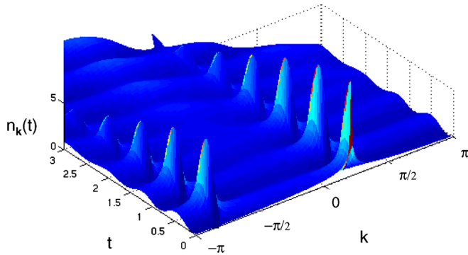
FIG. 3 (color online). n_k as a function of k and time for a boost of \nu = \pi/5 , superlattice strength V_0 = 4 , and hopping w = 1 . The initial peak is at k = \nu , and the peak transports back and forth to -4\pi/5 before disappearing due to decoherence. Results obtained using an exact diagonalization study of chains 150 sites long.
