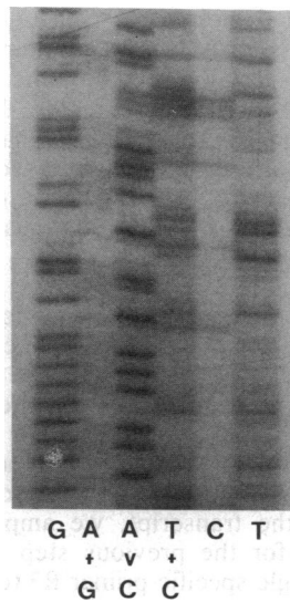
FIG. 3. Fragment of sequencing gel obtained by direct PCR-mediated method. The fragment shown corresponds to the internal core region of zebrafish tropomyosin cDNA (nucleotide positions 340–400). Sequencing reactions are as described in refs. 5 and 6.
