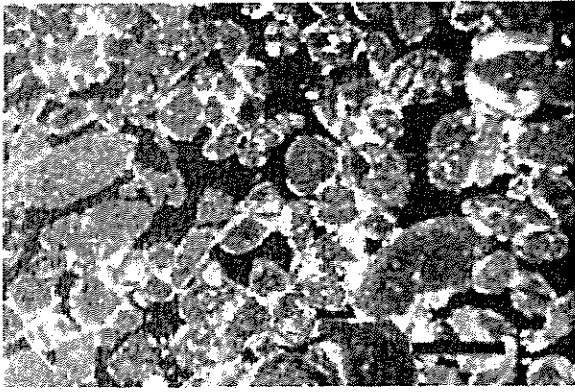
Figure 5: Meniscus calcite cement at grain contacts.
