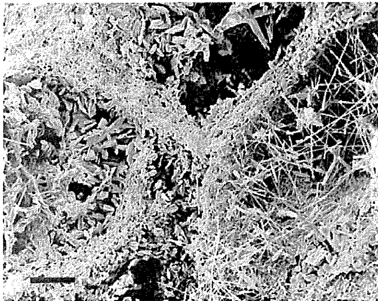
Figure 11: SEM photograph of whisker calcite and microsparite within pore space of alveolar texture.
