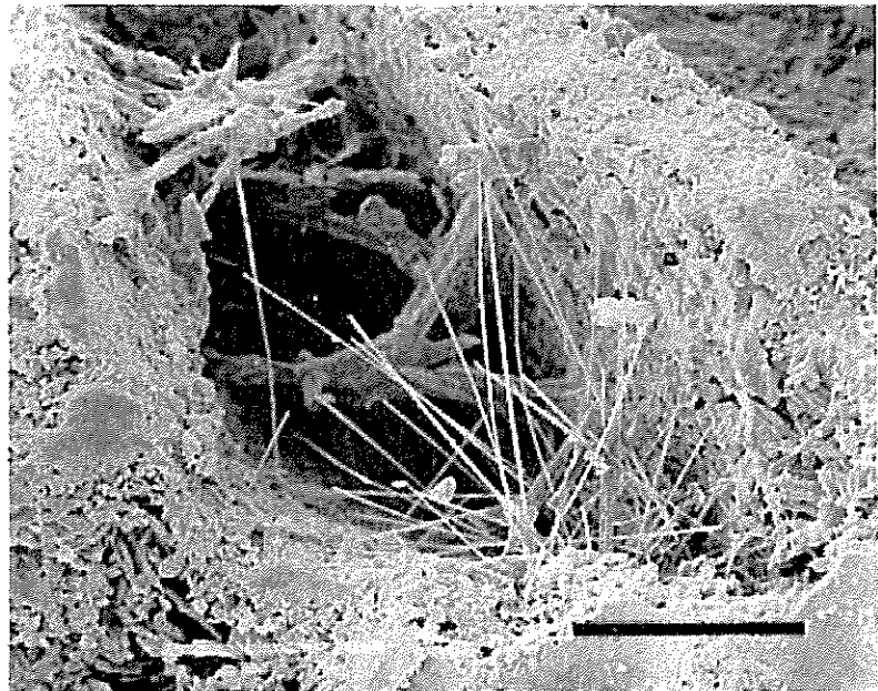
Figure 10: SEM photograph of whisker calcite within the pore space of alveolar texture.
