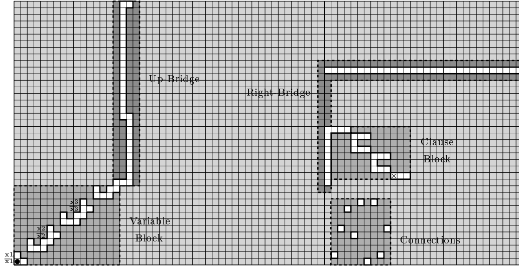
(b) Complete Example for the formula (x_1 \vee x_2 \vee x_3) \wedge (\overline{x_2} \vee x_3 \vee \overline{x_1}) \wedge (x_3 \vee x_1 \vee x_2) .
