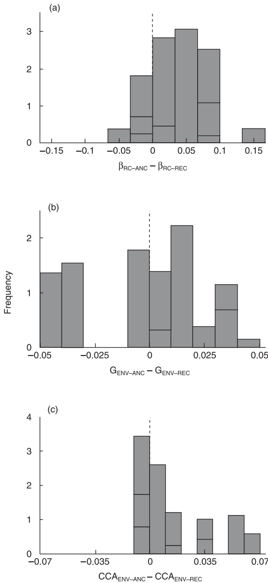
Fig. 1 Weighted histograms of the difference between ancient and recent forests for (a) the Raup-Crick measure of beta diversity for species \times site data, \beta_{RC} (b) Gower's dissimilarity coefficient for environmental data, G_{ENV} , and (c) the proportion of variation in community composition explained by environmental variables in a canonical correspondence analysis, CCA_{ENV} . In each histogram the summed height of the bars is equal to the number of studies included (11 in a, 10 in b and c), but each study is weighted according to the inverse of the variance of the mean difference between ancient and recent forests (see Methods for details).
